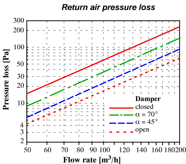
Pressure loss \Delta p selection diagram
