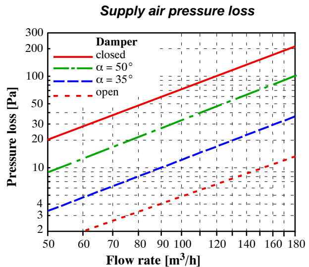
Damper setting
